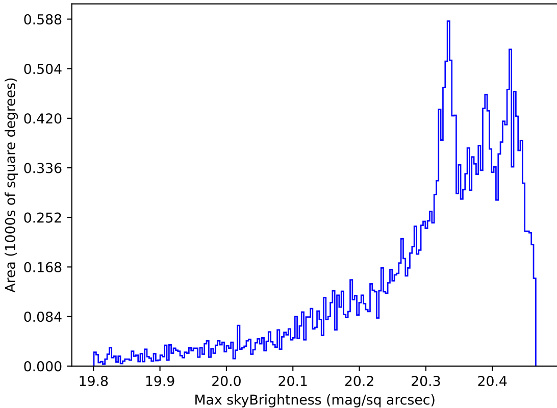
too_combined_s0.5_v3.4_10yrs All sky i band: Max skyBrightness
