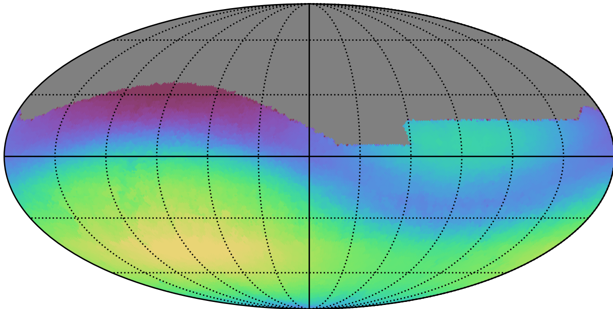
too_combined_s0.5_v3.4_10yrs All sky g band: Max skyBrightness
