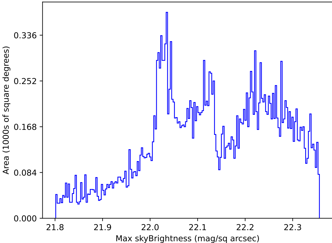
too_combined_s0.5_v3.4_10yrs All sky g band: Max skyBrightness
