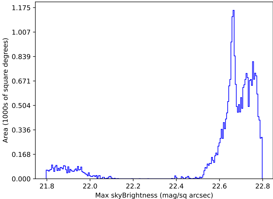
too_combined_s0.5_v3.4_10yrs All sky all bands: Max skyBrightness
