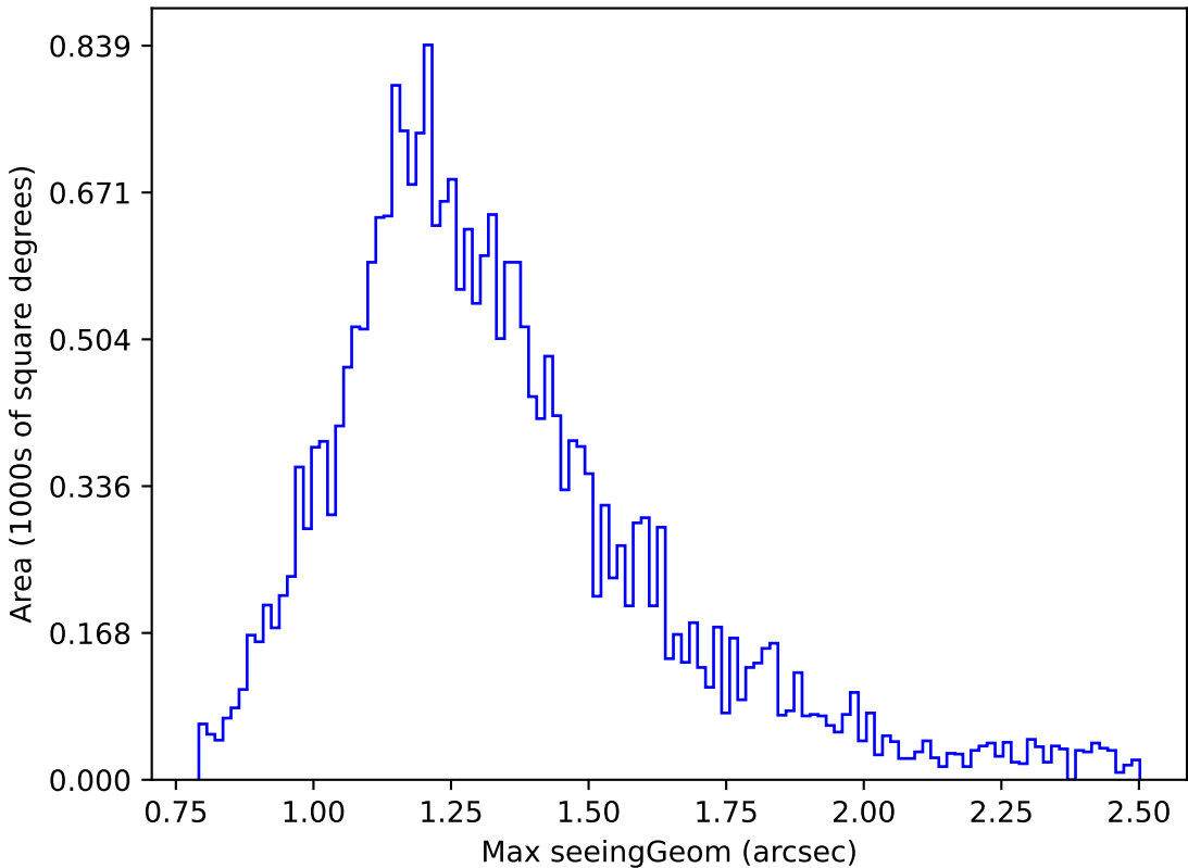
too_combined_s0.5_v3.4_10yrs Yr 1 z band: Max seeingGeom
