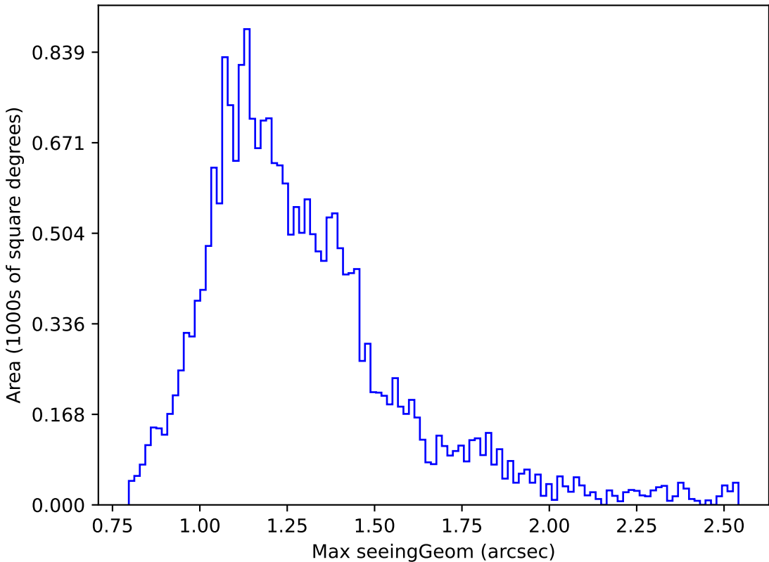
too_combined_s0.5_v3.4_10yrs Yr 1 y band: Max seeingGeom
