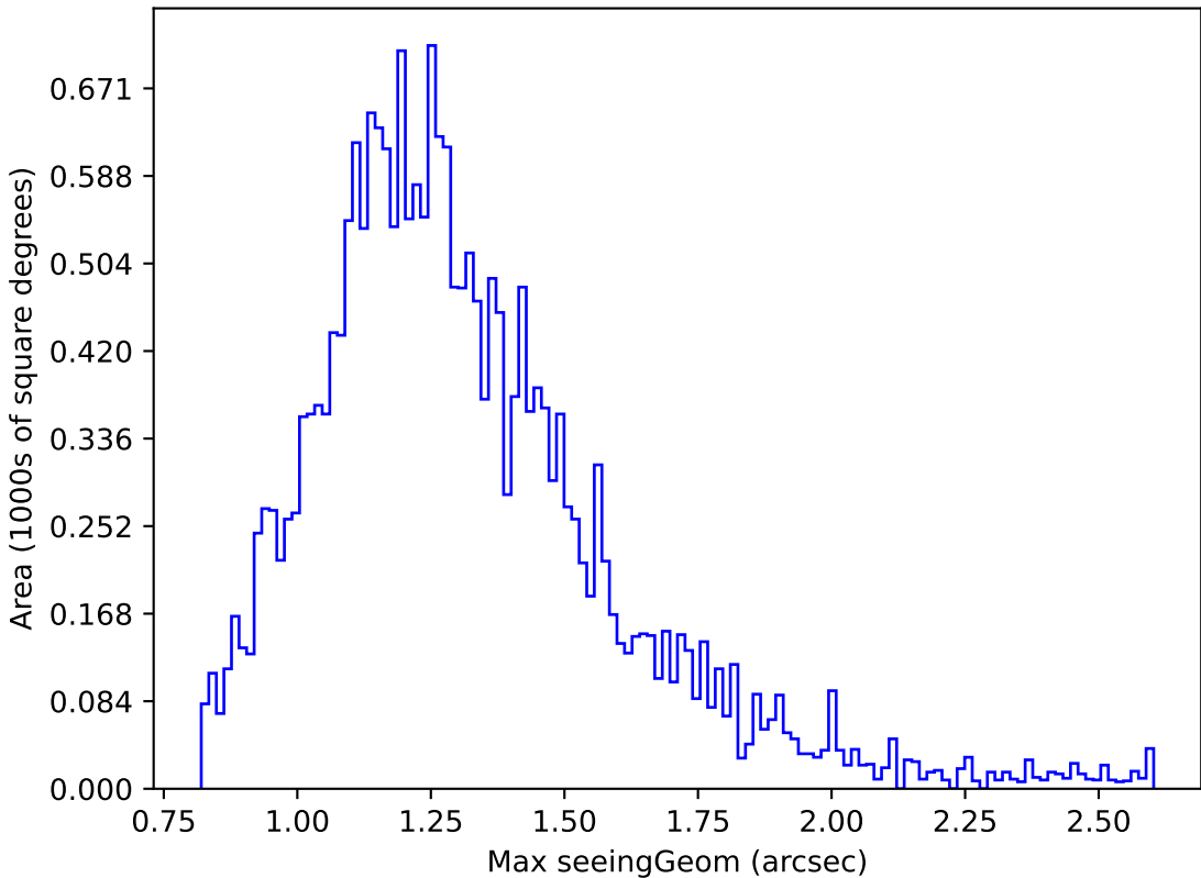
too_combined_s0.5_v3.4_10yrs Yr 1 u band: Max seeingGeom
