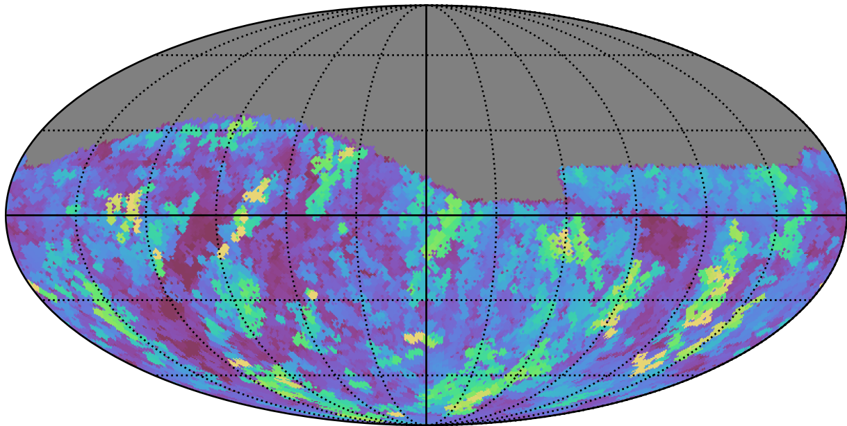
too_combined_s0.5_v3.4_10yrs Yr 1 r band: Max seeingGeom
