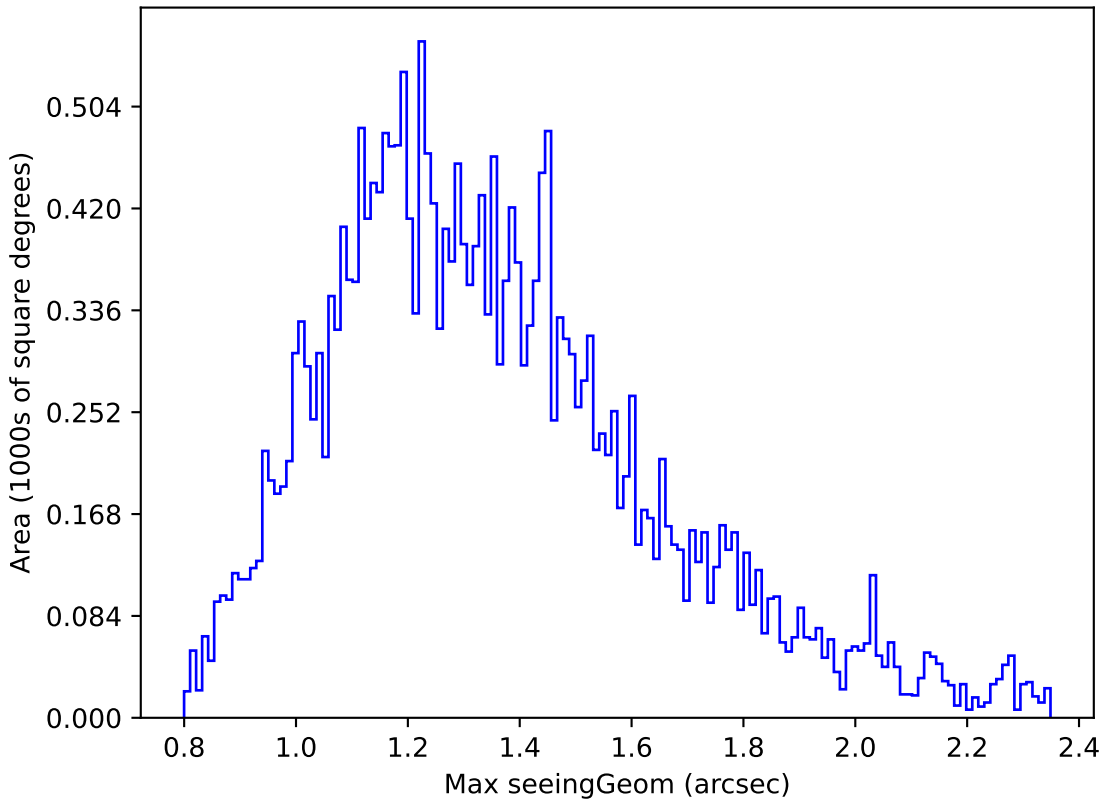
too_combined_s0.5_v3.4_10yrs Yr 1 r band: Max seeingGeom
