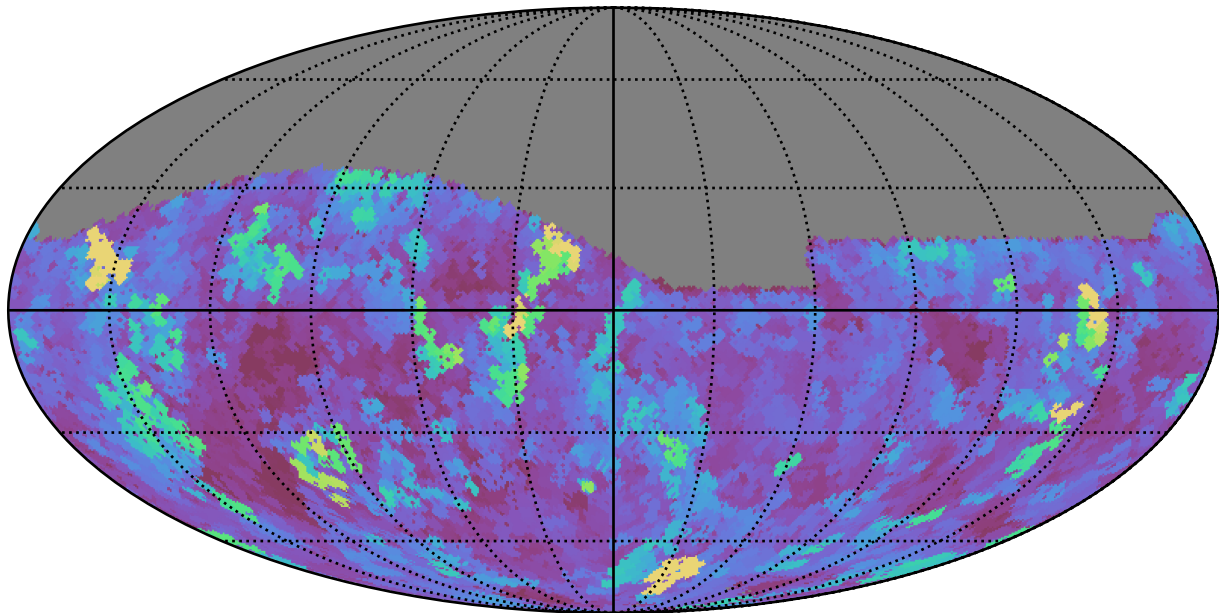
too_combined_s0.5_v3.4_10yrs Yr 1 i band: Max seeingGeom
