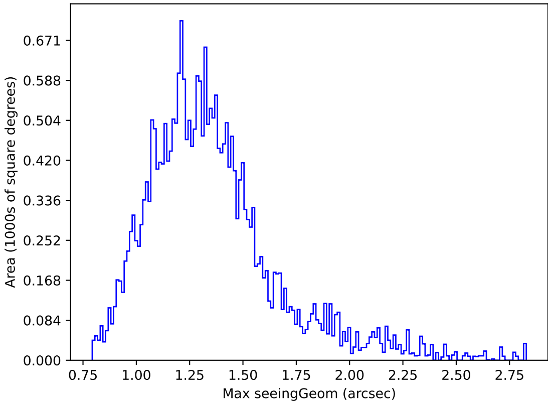
too_combined_s0.5_v3.4_10yrs Yr 1 i band: Max seeingGeom
