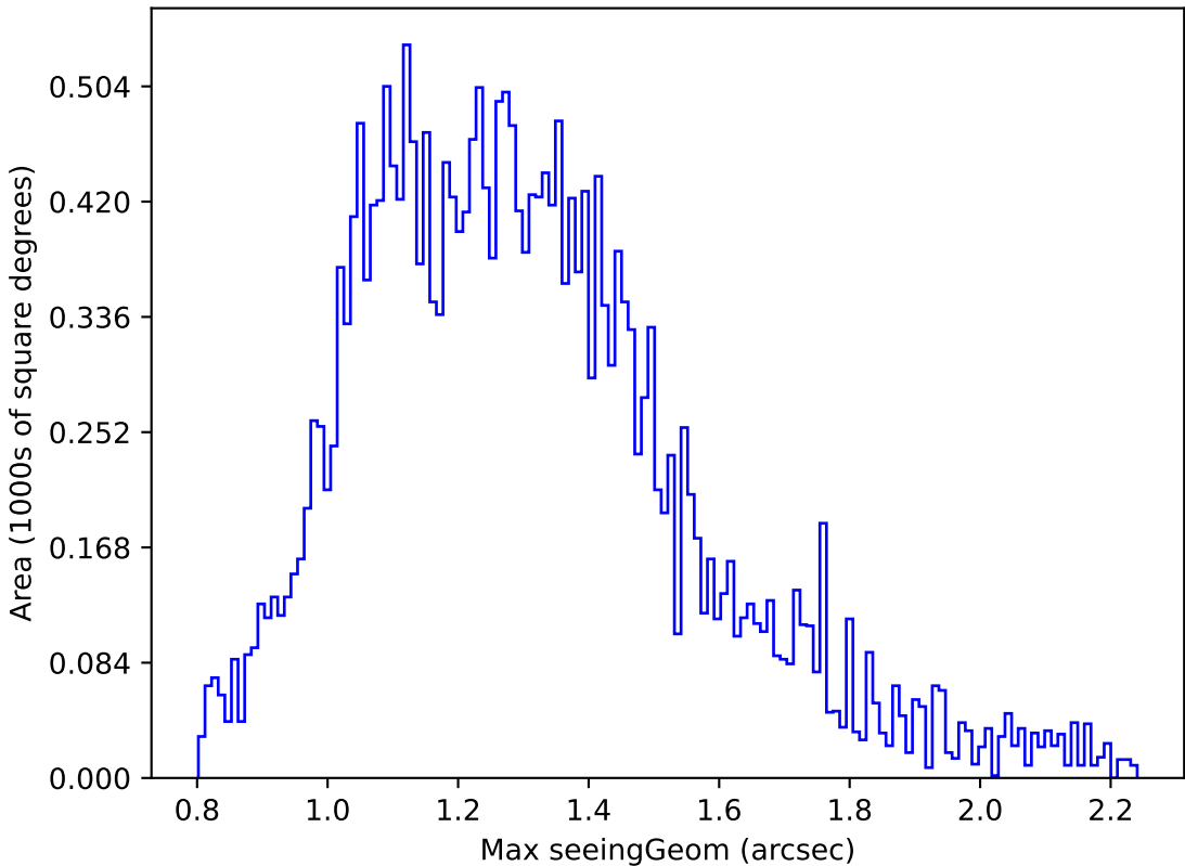
too_combined_s0.5_v3.4_10yrs Yr 1 g band: Max seeingGeom
