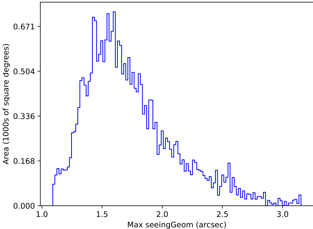
too_combined_s0.5_v3.4_10yrs Yr 1 all bands: Max seeingGeom
