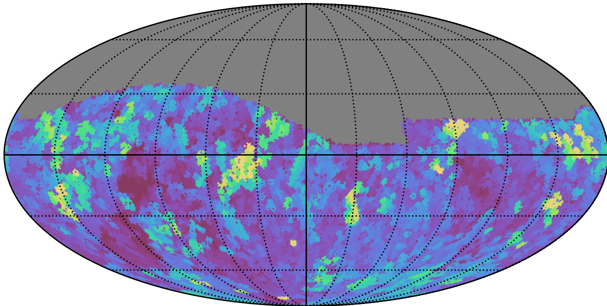
too_combined_s0.5_v3.4_10yrs Yr 1 z band: Max seeingEff
