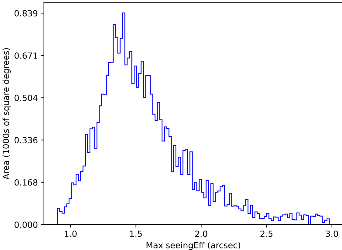
too_combined_s0.5_v3.4_10yrs Yr 1 z band: Max seeingEff
