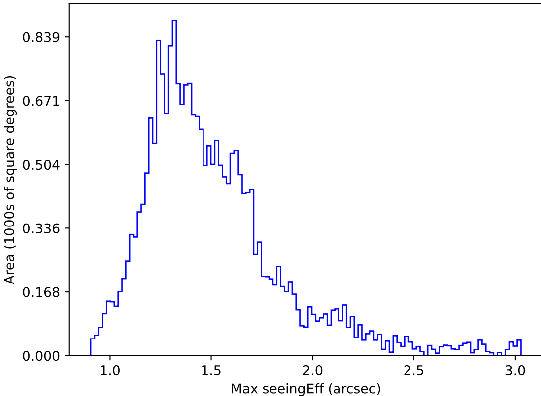
too_combined_s0.5_v3.4_10yrs Yr 1 y band: Max seeingEff
