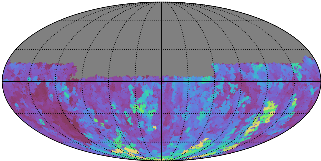
too_combined_s0.5_v3.4_10yrs Yr 1 u band: Max seeingEff
