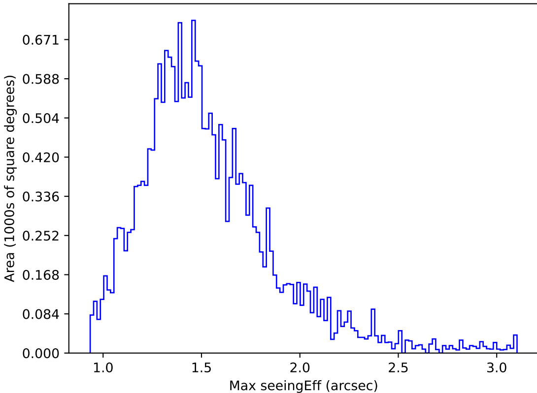
too_combined_s0.5_v3.4_10yrs Yr 1 u band: Max seeingEff
