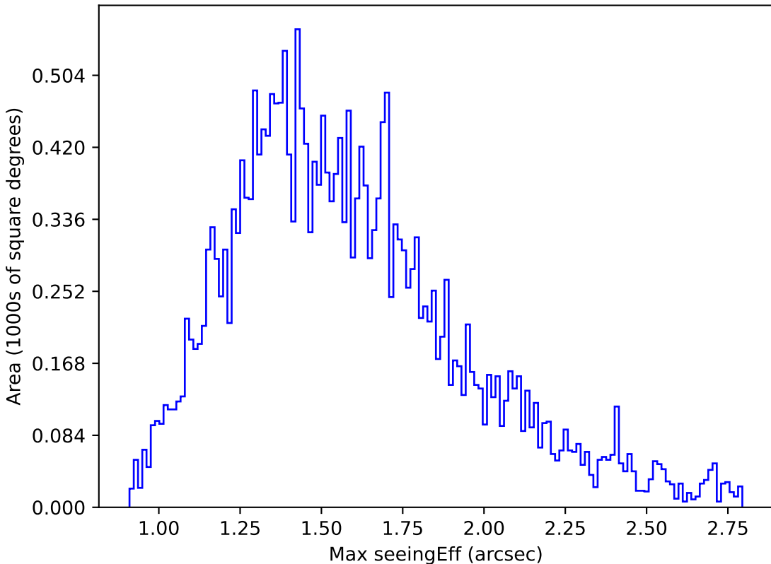
too_combined_s0.5_v3.4_10yrs Yr 1 r band: Max seeingEff
