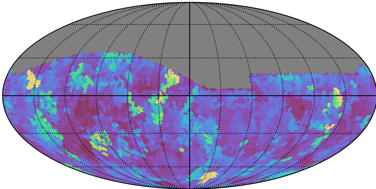
too_combined_s0.5_v3.4_10yrs Yr 1 i band: Max seeingEff
