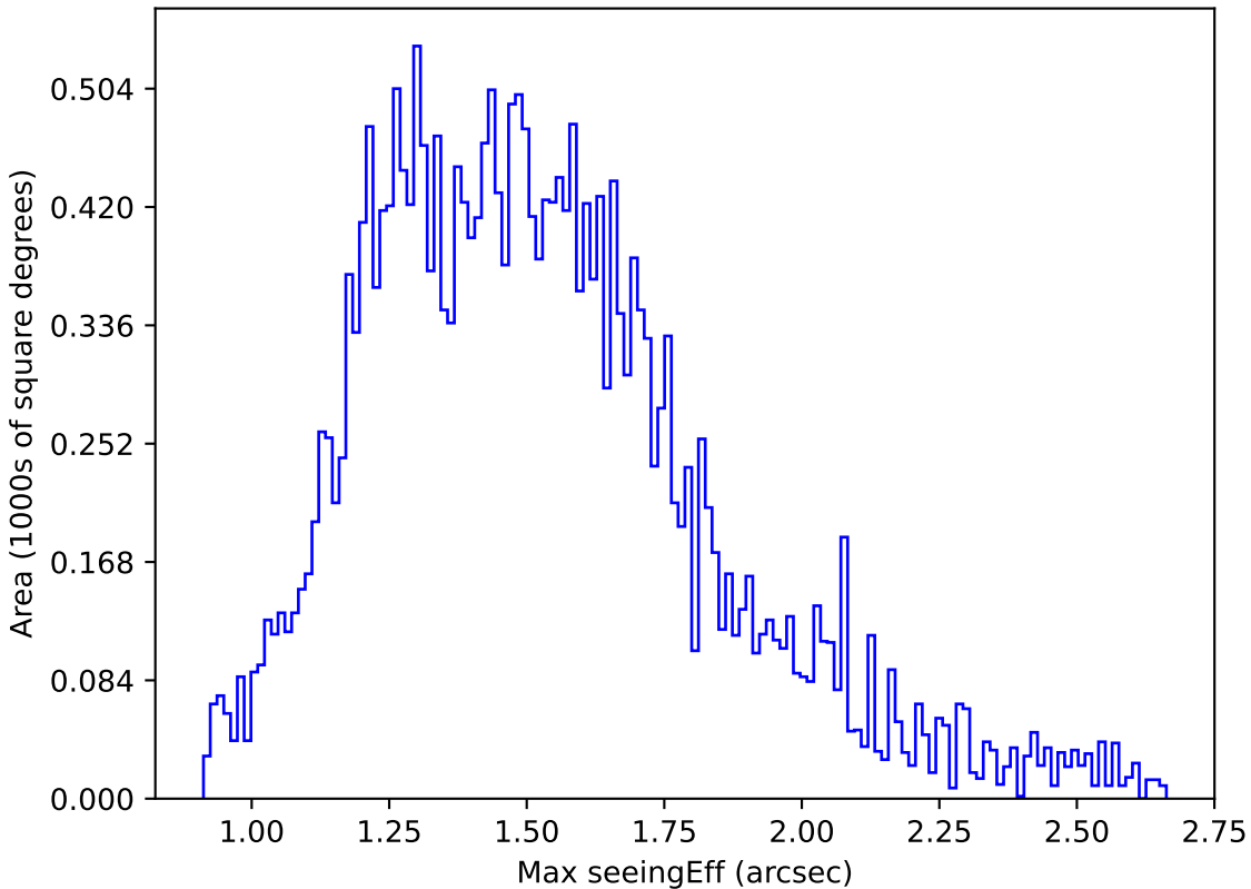
too_combined_s0.5_v3.4_10yrs Yr 1 g band: Max seeingEff
