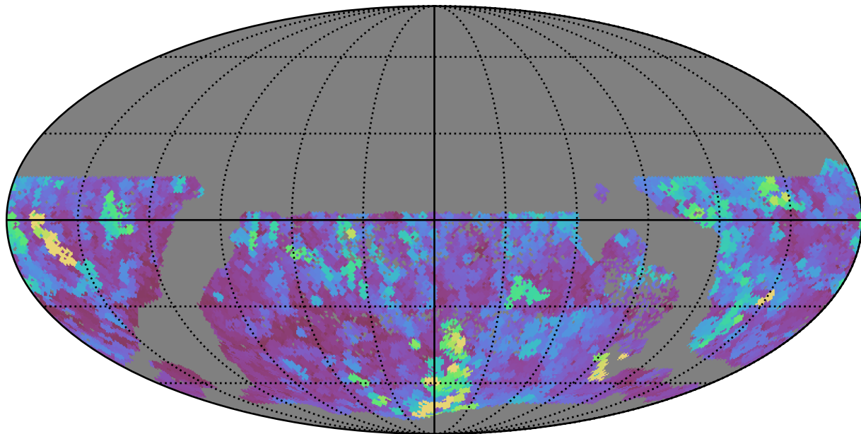
too_combined_s0.5_v3.4_10yrs WFD z band: Max seeingEff
