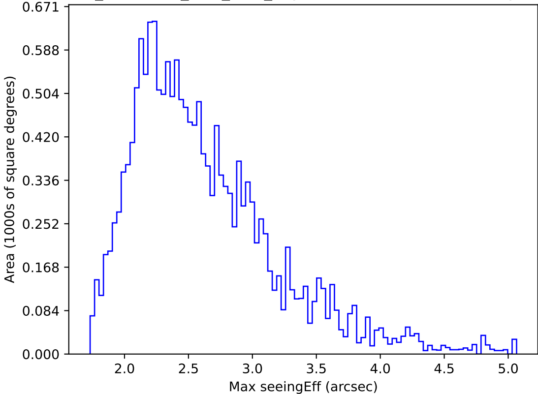
too_combined_s0.5_v3.4_10yrs WFD z band: Max seeingEff
