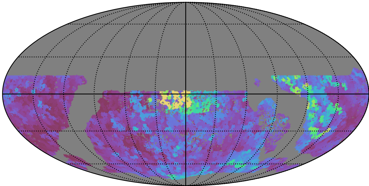
too_combined_s0.5_v3.4_10yrs WFD y band: Max seeingEff
