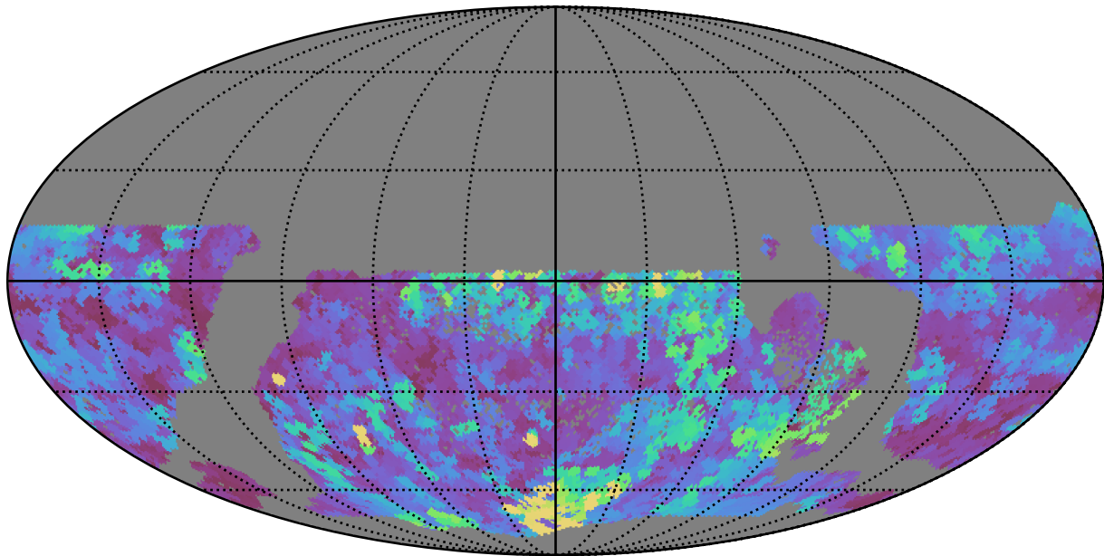
too_combined_s0.5_v3.4_10yrs WFD u band: Max seeingEff
