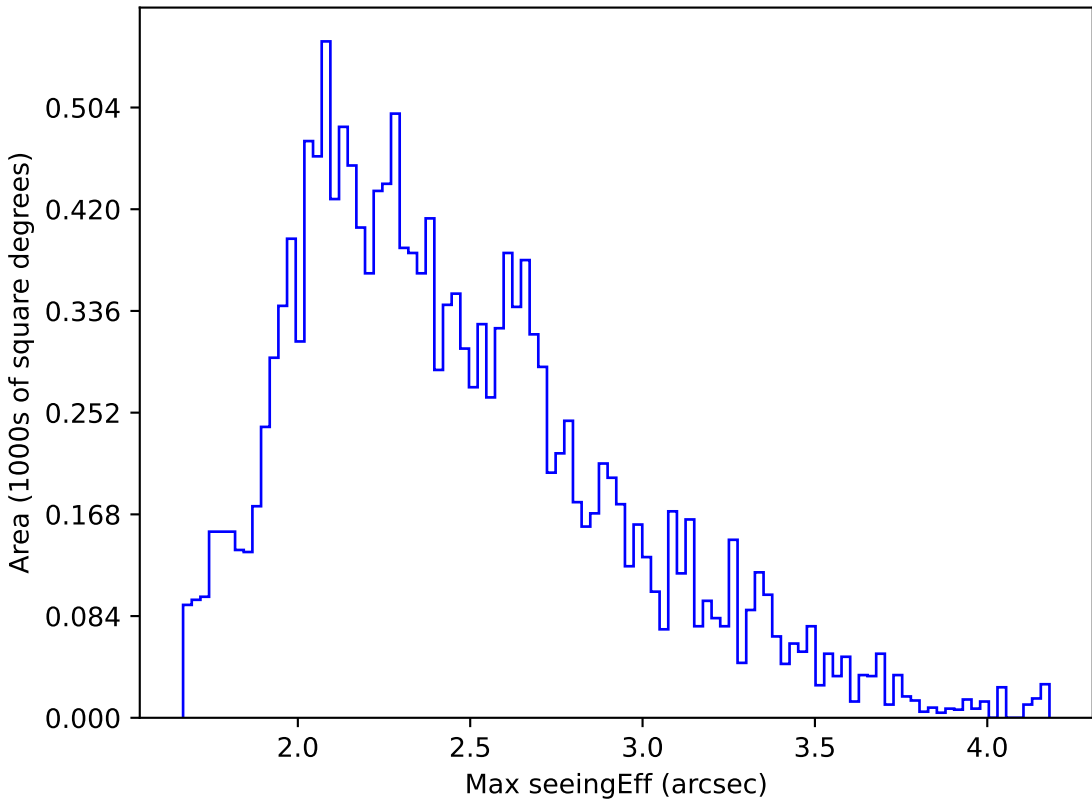
too_combined_s0.5_v3.4_10yrs WFD u band: Max seeingEff
