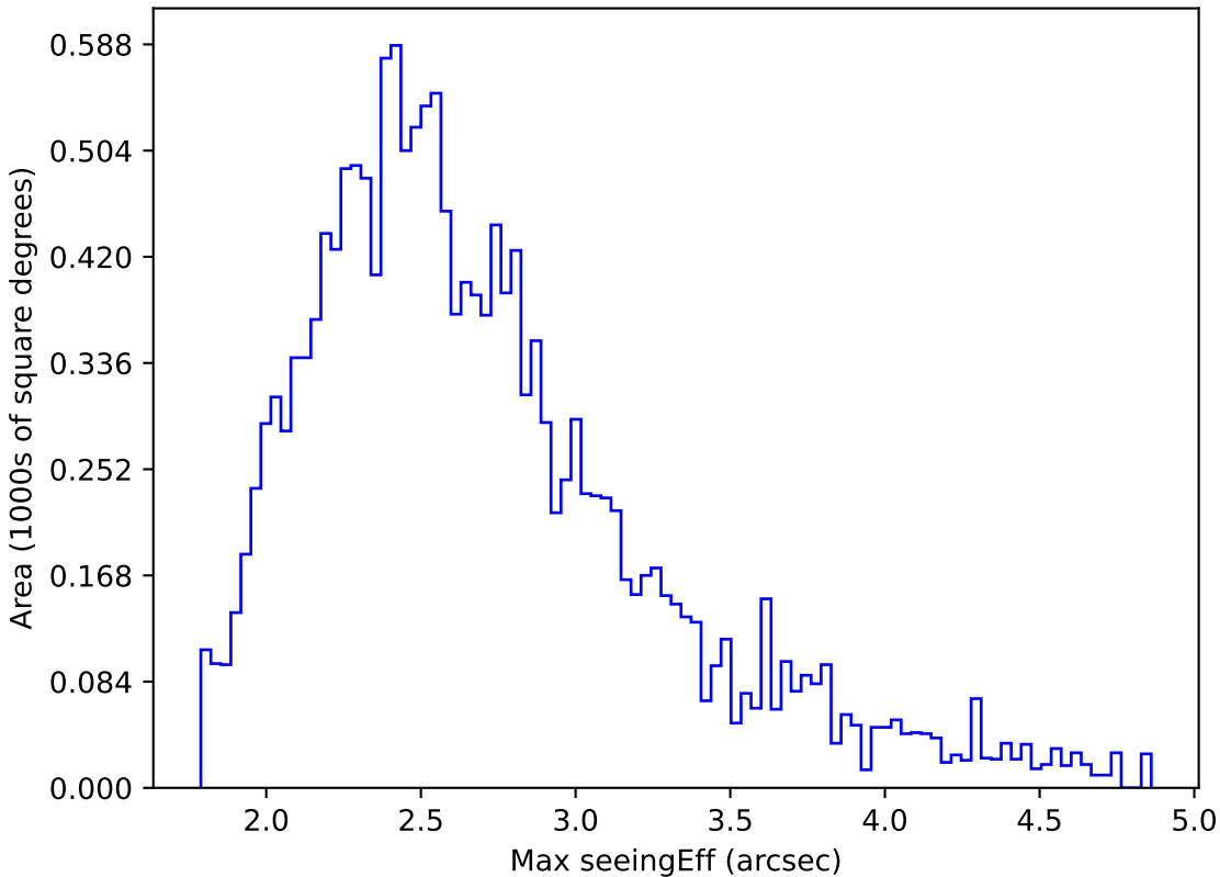
too_combined_s0.5_v3.4_10yrs WFD i band: Max seeingEff
