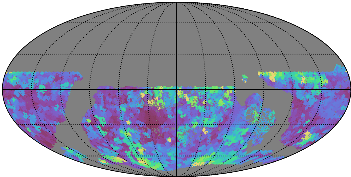
too_combined_s0.5_v3.4_10yrs WFD g band: Max seeingEff
