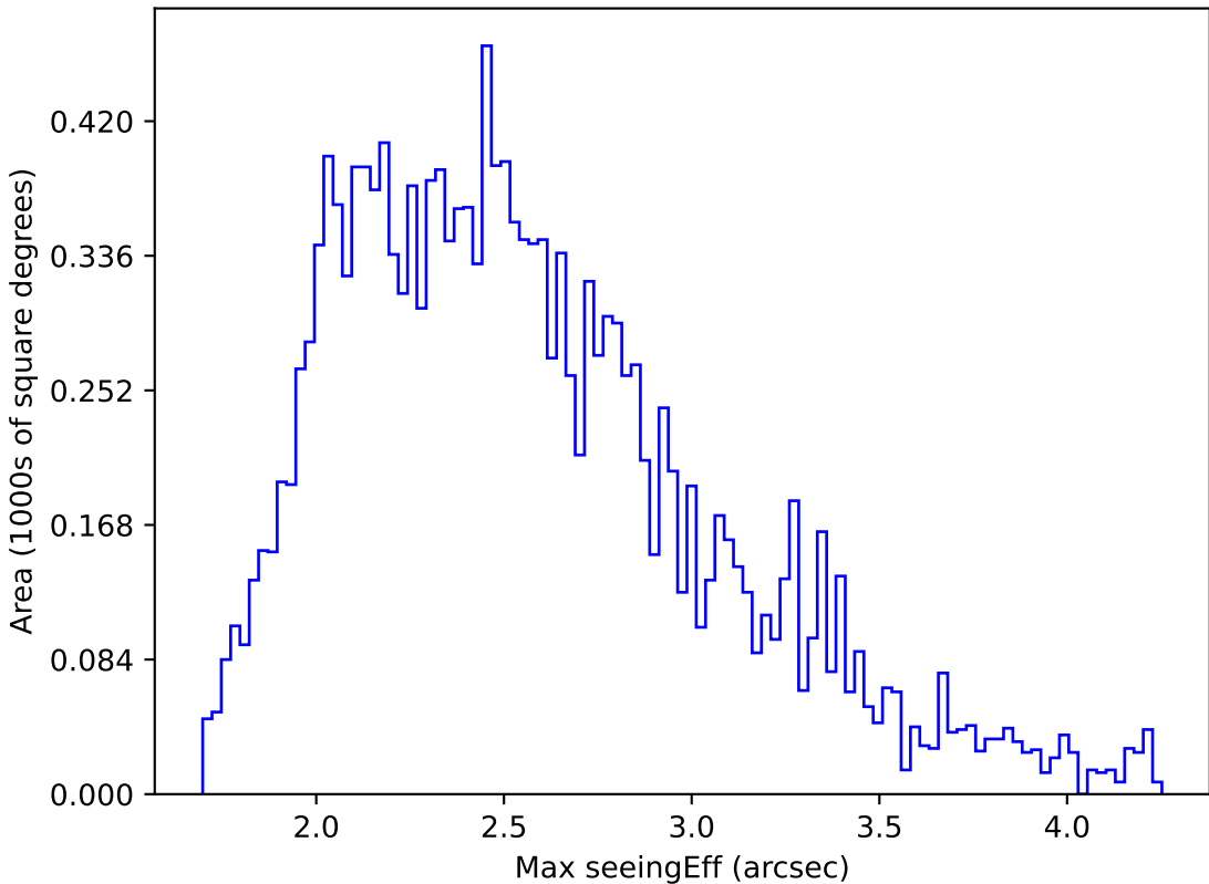
too_combined_s0.5_v3.4_10yrs WFD g band: Max seeingEff
