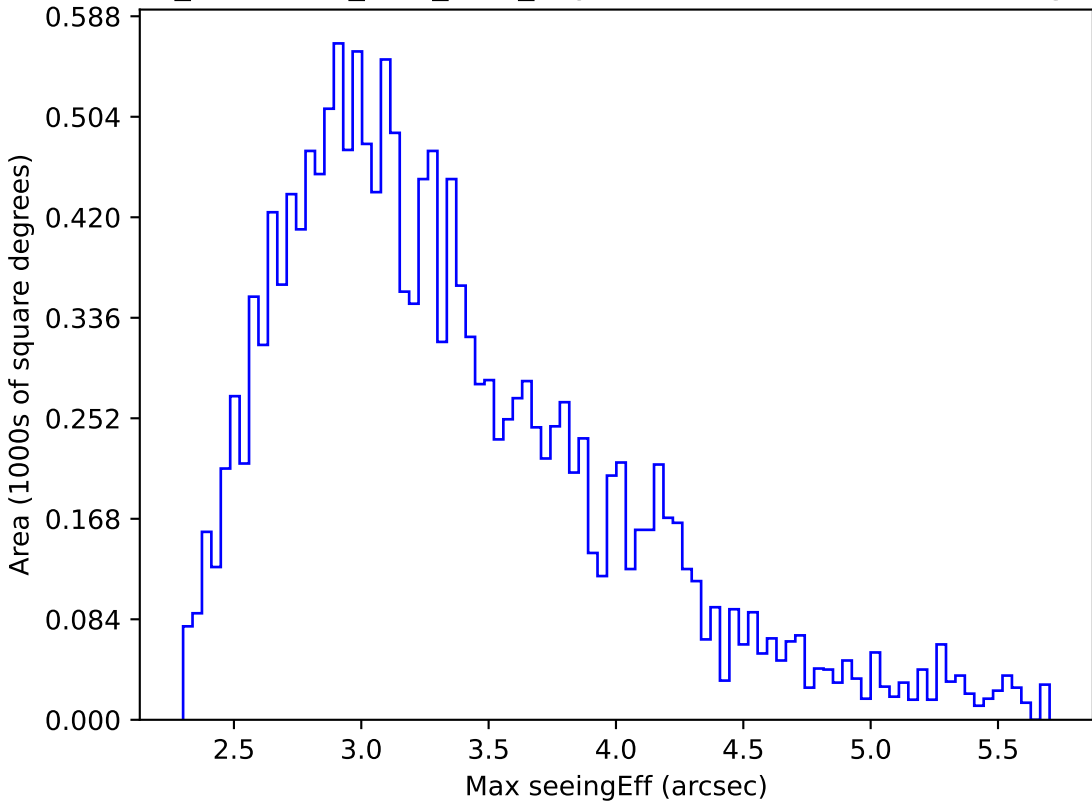
too_combined_s0.5_v3.4_10yrs WFD all bands: Max seeingEff
