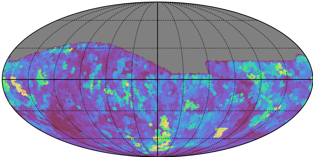
too_combined_s0.5_v3.4_10yrs All sky z band: Max seeingEff
