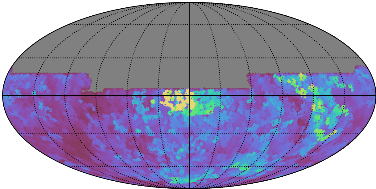
too_combined_s0.5_v3.4_10yrs All sky y band: Max seeingEff
