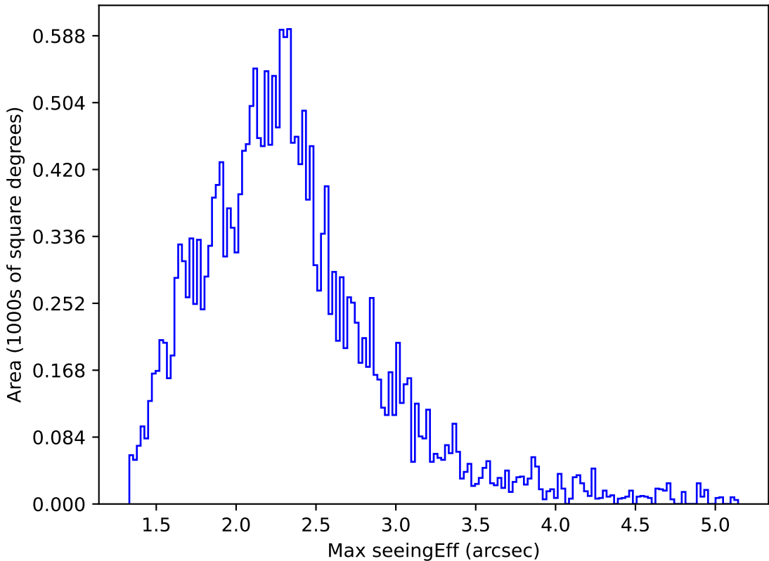
too_combined_s0.5_v3.4_10yrs All sky y band: Max seeingEff
