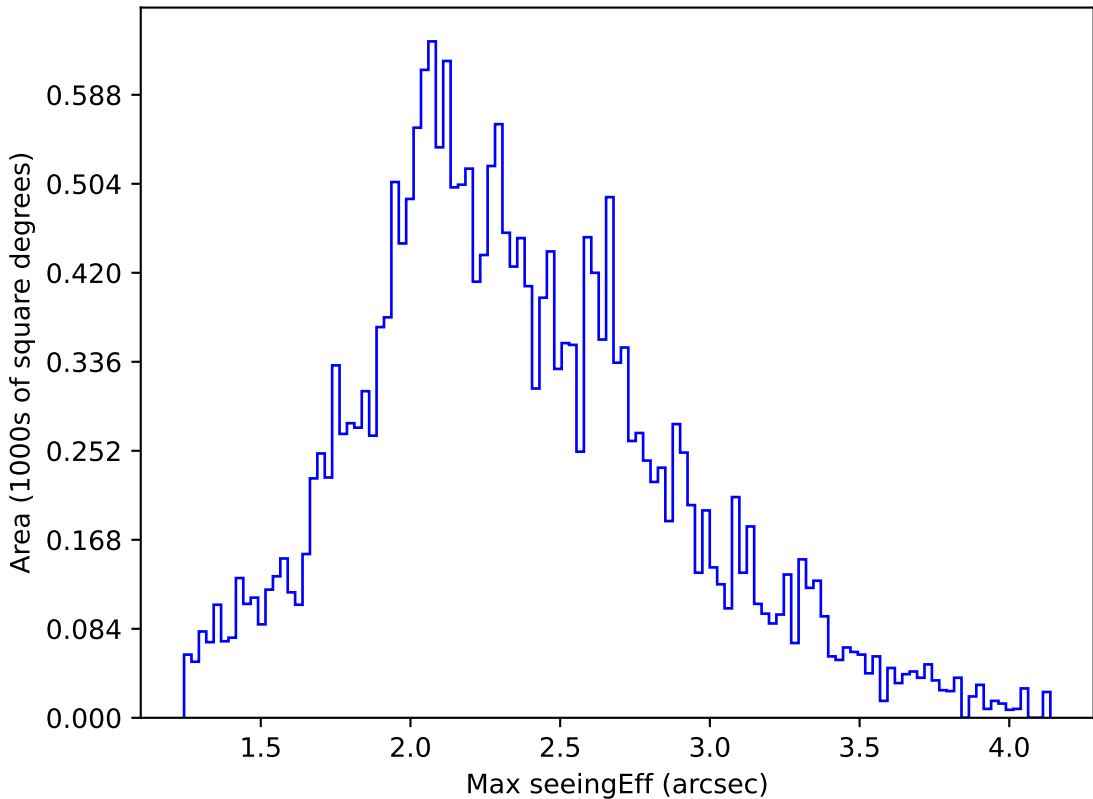
too_combined_s0.5_v3.4_10yrs All sky u band: Max seeingEff
