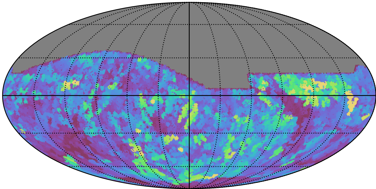
too_combined_s0.5_v3.4_10yrs All sky r band: Max seeingEff
