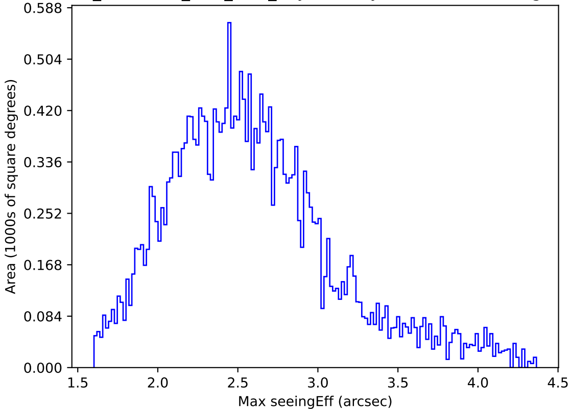
too_combined_s0.5_v3.4_10yrs All sky r band: Max seeingEff
