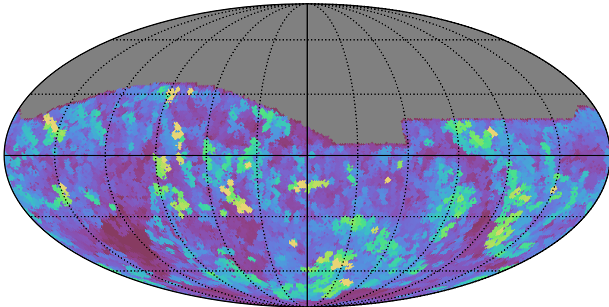
too_combined_s0.5_v3.4_10yrs All sky i band: Max seeingEff
