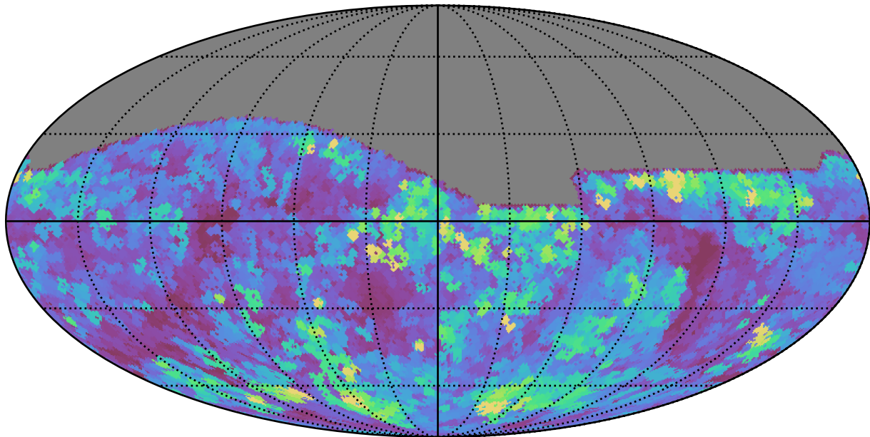
too_combined_s0.5_v3.4_10yrs All sky g band: Max seeingEff
