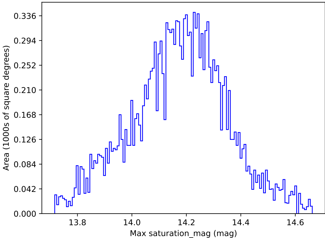
too_combined_s0.5_v3.4_10yrs WFD y band: Max saturation_mag
