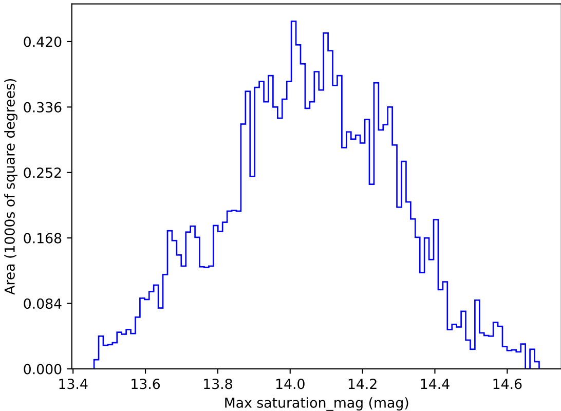
too_combined_s0.5_v3.4_10yrs WFD u band: Max saturation_mag
