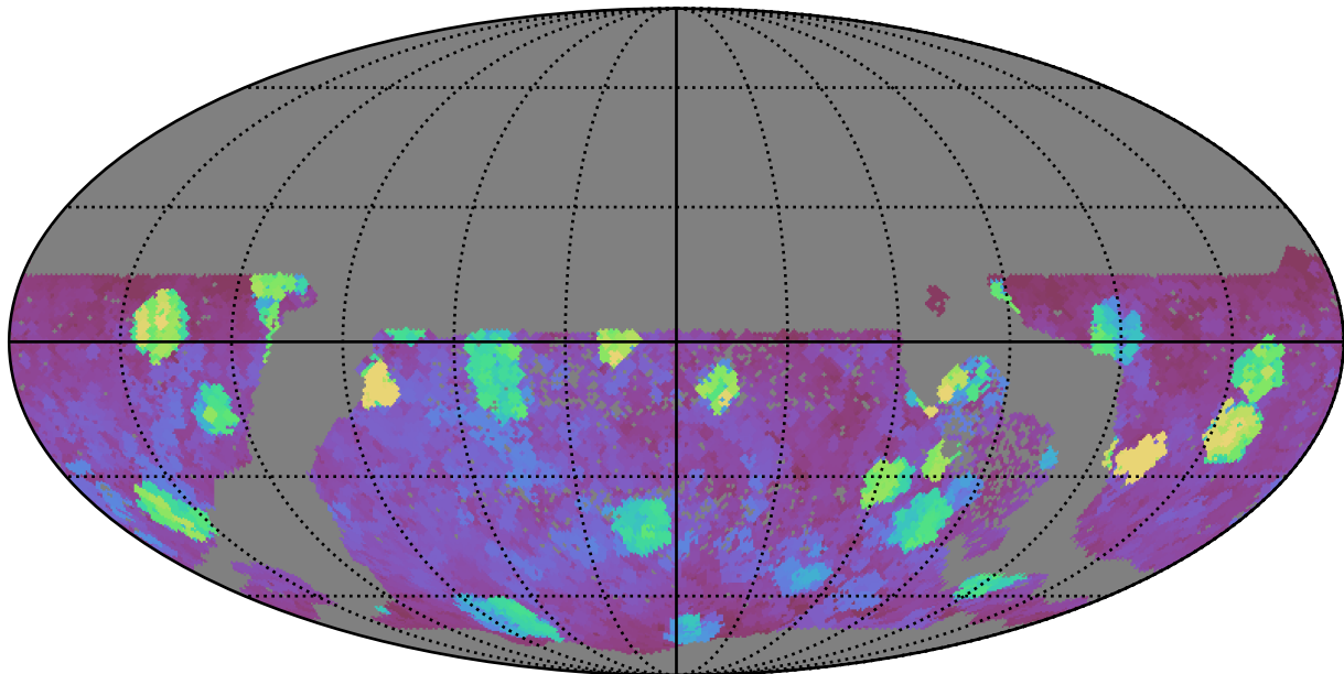
too_combined_s0.5_v3.4_10yrs WFD i band: Max saturation_mag
