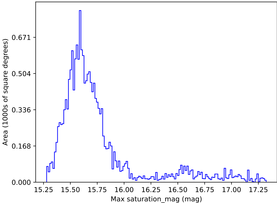
too_combined_s0.5_v3.4_10yrs WFD i band: Max saturation_mag
