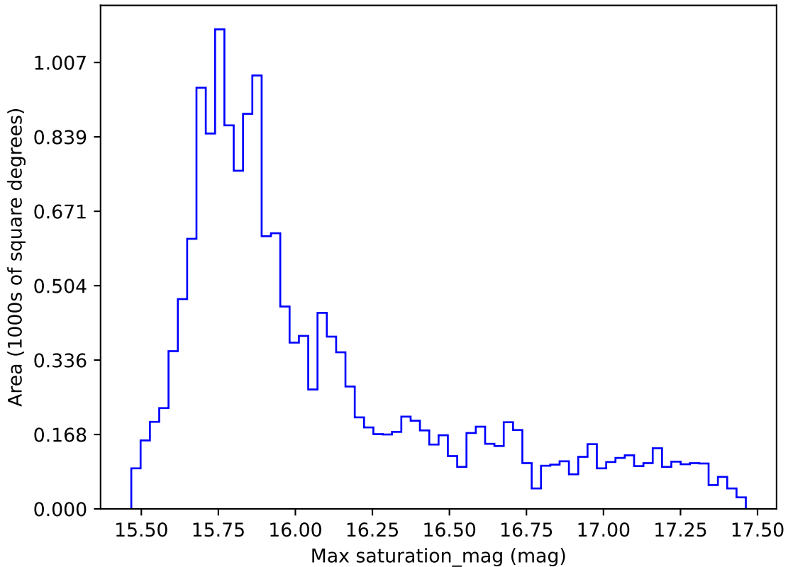
too_combined_s0.5_v3.4_10yrs WFD all bands: Max saturation_mag
