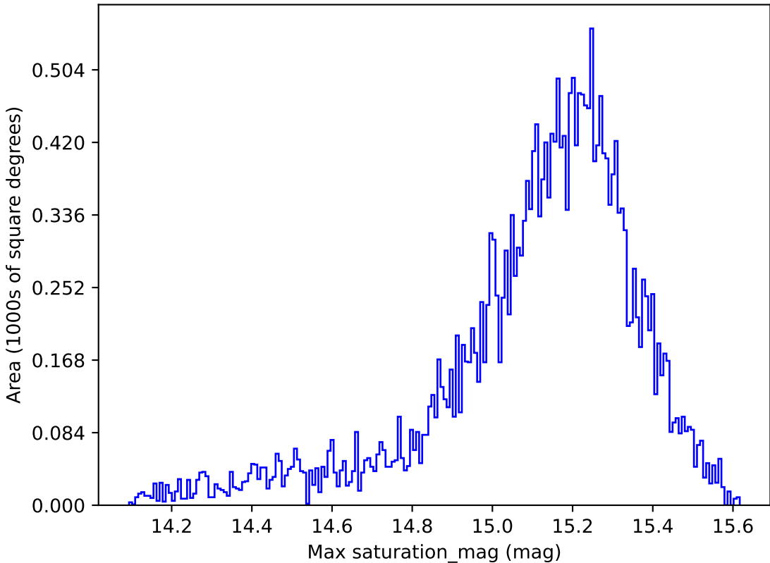
too_combined_s0.5_v3.4_10yrs All sky z band: Max saturation_mag
