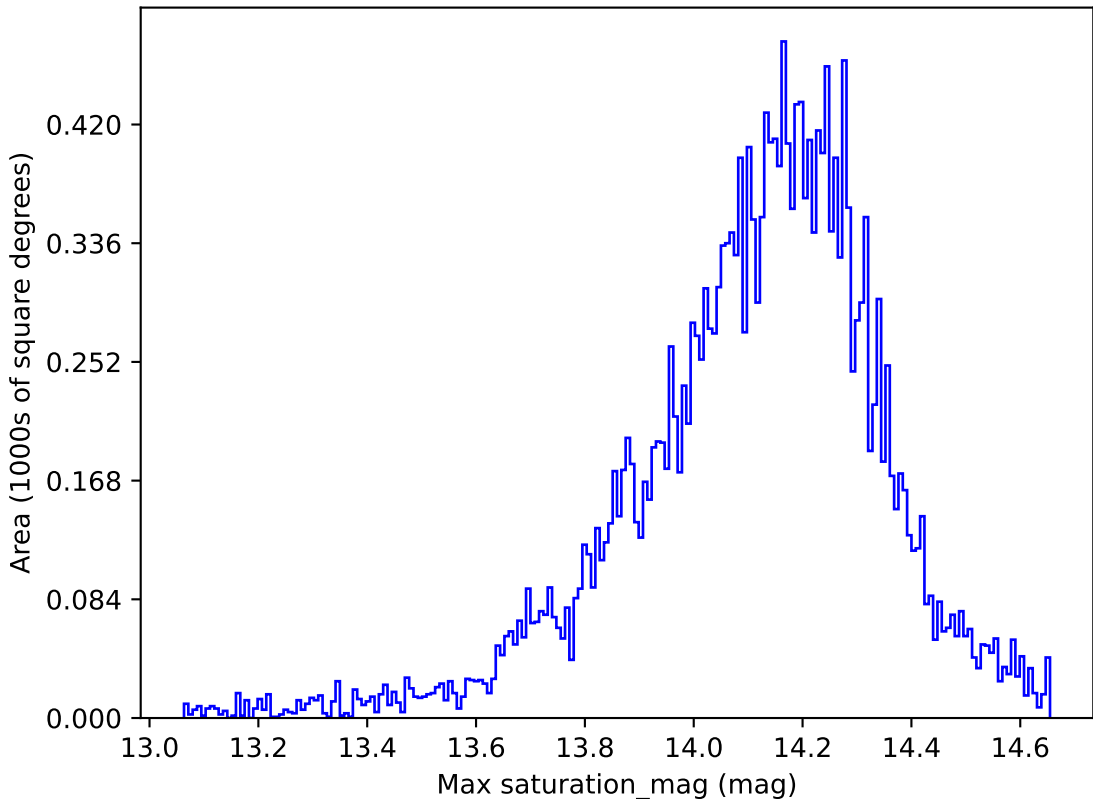
too_combined_s0.5_v3.4_10yrs All sky y band: Max saturation_mag
