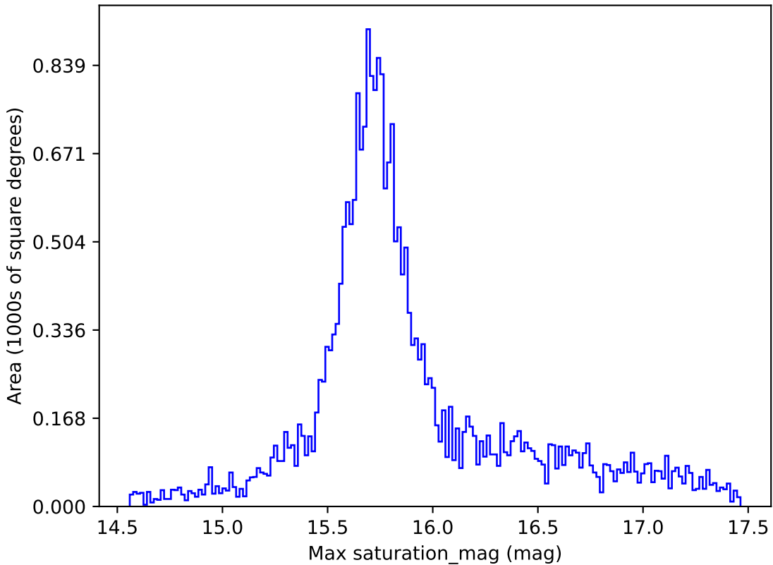
too_combined_s0.5_v3.4_10yrs All sky r band: Max saturation_mag
