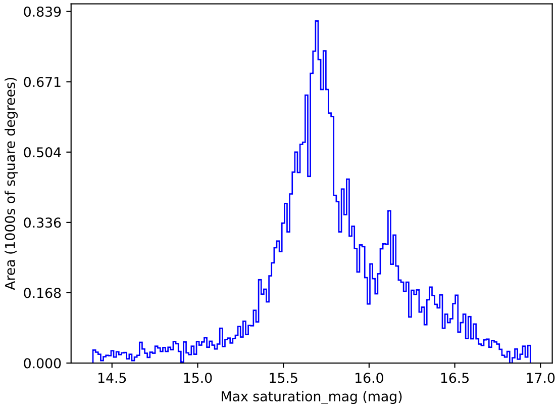
too_combined_s0.5_v3.4_10yrs All sky g band: Max saturation_mag
