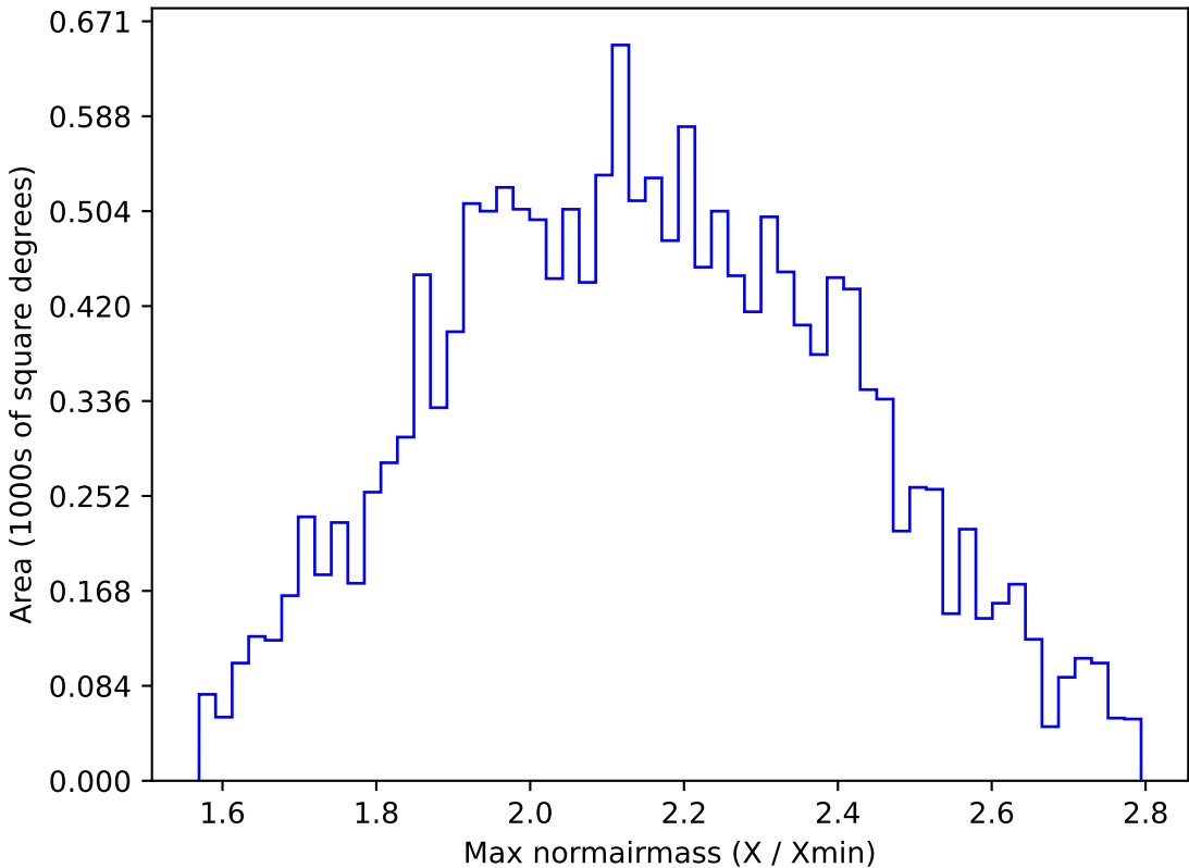
too_combined_s0.5_v3.4_10yrs WFD y band: Max normairmass
