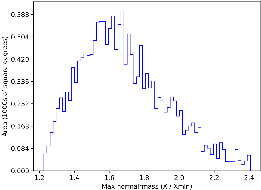
too_combined_s0.5_v3.4_10yrs WFD u band: Max normairmass
