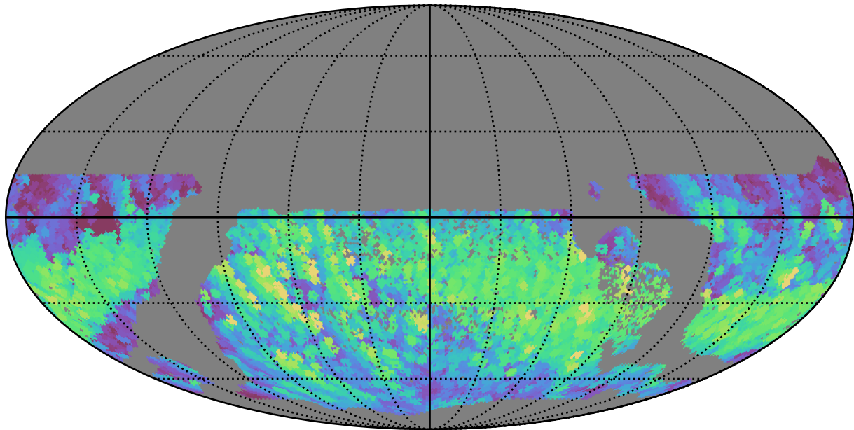
too_combined_s0.5_v3.4_10yrs WFD r band: Max normairmass
